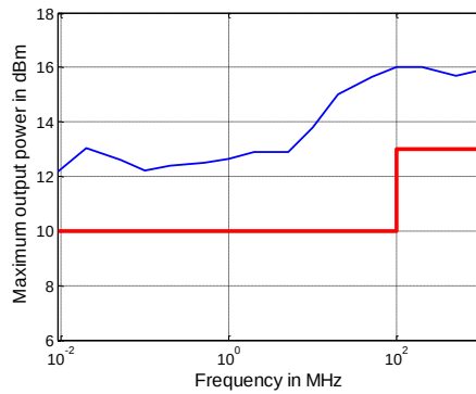
Maximum output power in dBm versus frequency of the R&amp;S®ZNB8
