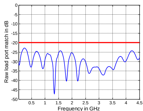
Raw load port match versus frequency of the R&S®ZNB4
