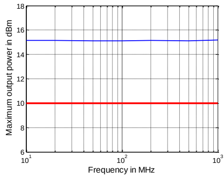
Maximum output power in dBm versus frequency of the R&S®ZNB40 model .72
