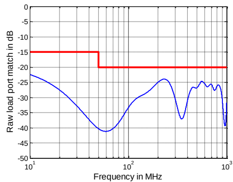
Raw load port match versus frequency of the R&amp;S®ZNB40 model .72
