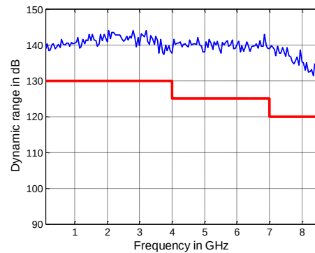
Dynamic range in dB versus frequency of the R&amp;S®ZNB8
