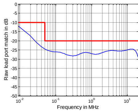
Raw load port match versus frequency of the R&amp;S®ZNB8
