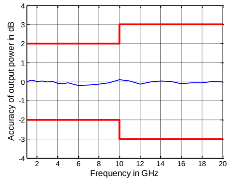
Output power accuracy in dB versus frequency of the R&S®ZNB20
