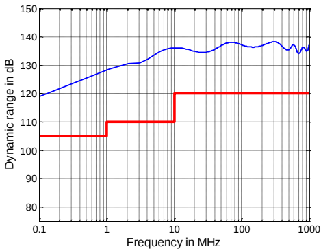
Dynamic range in dB versus frequency of the R&S®ZNB40 models .82 and .84
