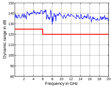
Dynamic range in dB versus frequency of the R&S®ZNB20
