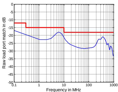
Raw load port match versus frequency of the R&amp;S®ZNB40 models .82 and .84
