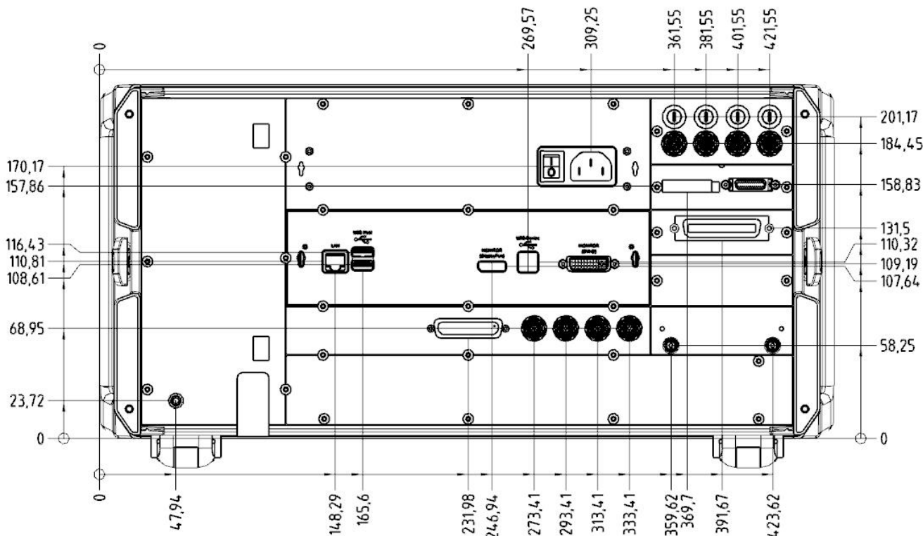
Rear view of the R&S®ZNB
