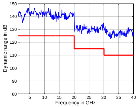
Dynamic range in dB versus frequency of the R&S®ZNB40 model .72
