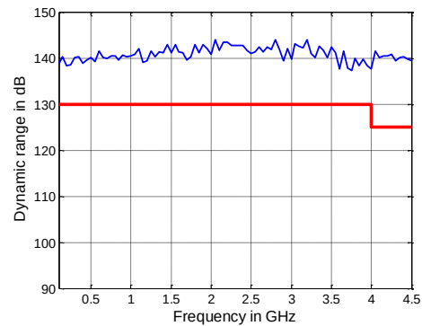
Dynamic range in dB versus frequency of the R&amp;S®ZNB4
