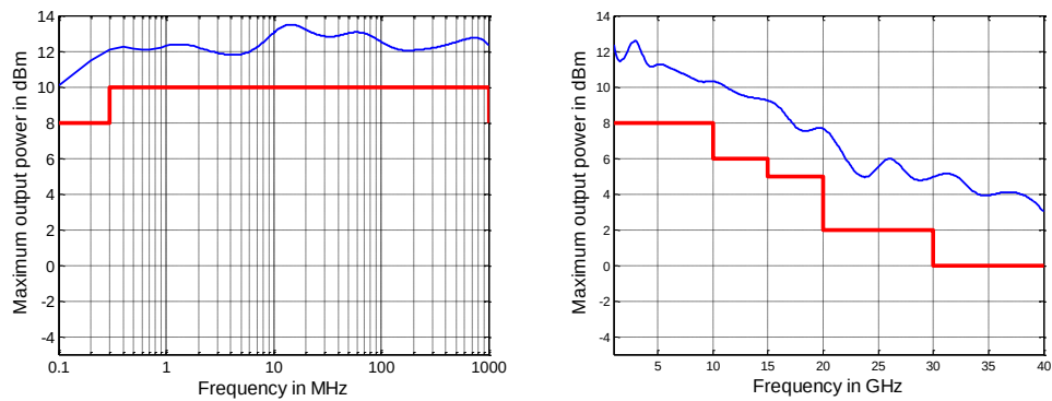
Maximum output power in dBm versus frequency of the R&S®ZNB40 models .82 and .84
