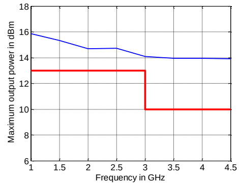
Maximum output power in dBm versus frequency of the R&amp;S®ZNB4
