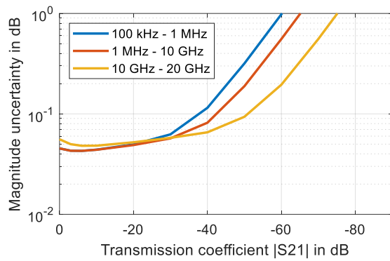
Uncertainty of transmission magnitude and transmission phase measurements of the R&S®ZNB20 in the frequency range from 100 kHz to 20 GHz; analysis conditions: S_{11} = S_{22} = 0 , cal. power -10 dBm, meas. power -10 dBm
