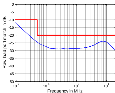
Raw load port match versus frequency of the R&S®ZNB4
