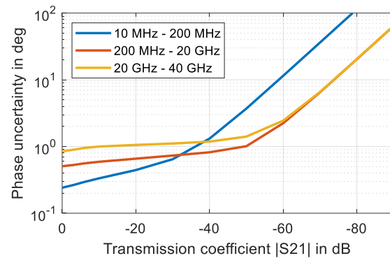
Uncertainty of transmission magnitude and transmission phase measurements of the R&S®ZNB40 model .72 in the frequency range from 10 MHz to 40 GHz; analysis conditions: S_{11} = S_{22} = 0 , cal. power –10 dBm, meas. power –10 dBm
