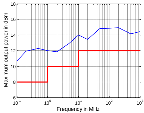
Maximum output power in dBm versus frequency of the R&S®ZNB20
