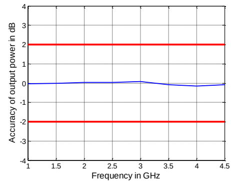
Output power accuracy in dB versus frequency of the R&amp;S®ZNB4
