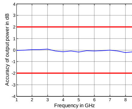
Output power accuracy in dB versus frequency of the R&amp;S®ZNB8
