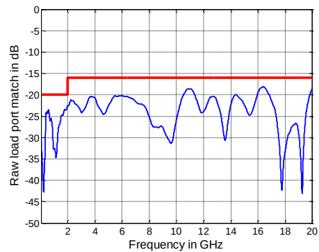
Raw load port match versus frequency of the R&amp;S®ZNB20
