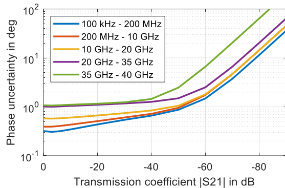
Uncertainty of transmission magnitude and transmission phase measurements of the R&S®ZNB40 models .82 and .84 in the frequency range from 100 kHz to 40 GHz; analysis conditions: S_{11} = S_{22} = 0 , cal. power -10 dBm, meas. power -10 dBm
