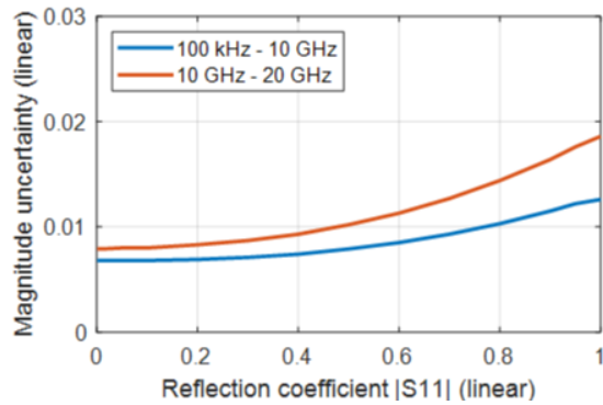
Uncertainty of reflection magnitude and reflection phase measurements of the R&S®ZNB20 in the frequency range from 100 kHz to 20 GHz; analysis conditions: S_{12} = S_{21} = 0 , cal. power -10 dBm, meas. power -10 dBm
