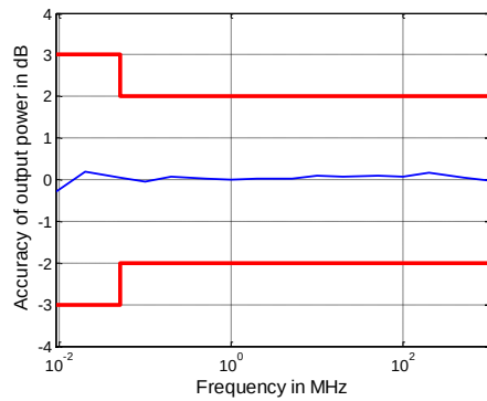
Output power accuracy in dB versus frequency of the R&amp;S®ZNB4
