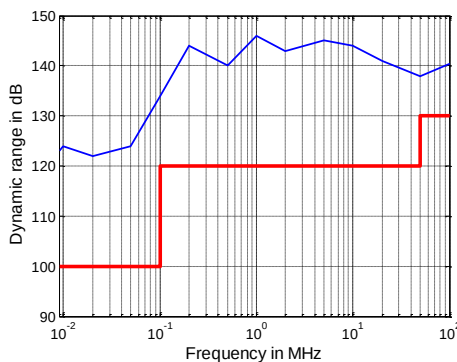
Dynamic range in dB versus frequency of the R&amp;S®ZNB8
