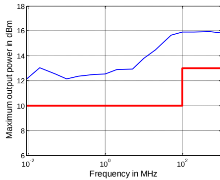
Maximum output power in dBm versus frequency of the R&amp;S®ZNB4
