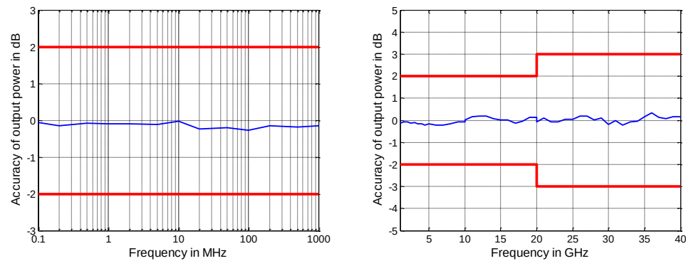
Output power accuracy in dB versus frequency of the R&S®ZNB40 models .82 and .84
