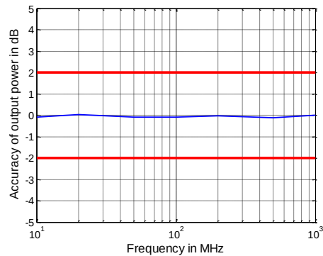
Output power accuracy in dB versus frequency of the R&S®ZNB40 model .72
